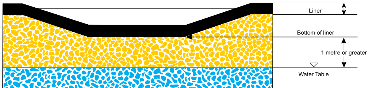
Figure 2 - Water Table Depth Requirement for Compacted Soil Liner
