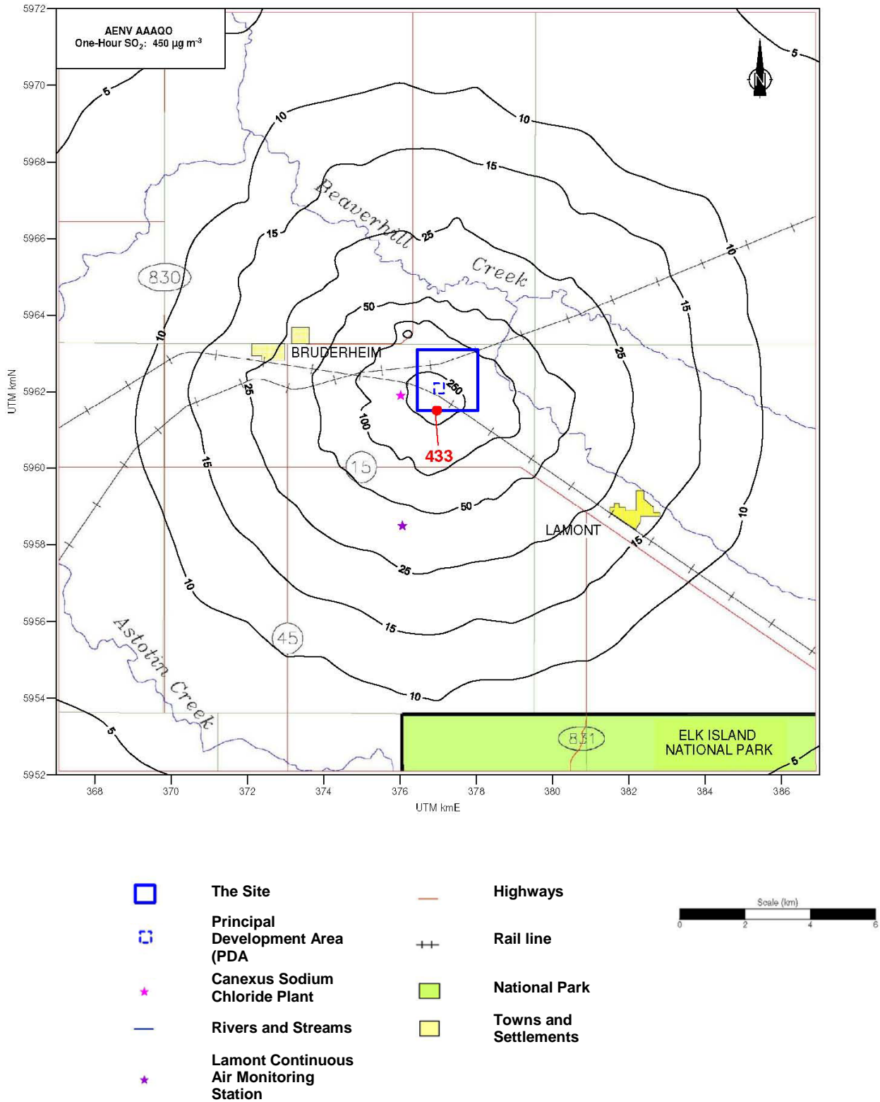
Figure 2.5-15: Isopleths of Maximum Predicted Hourly Average Ground-level SO 2 Concentrations (µg m -3 ) associated with Emissions from the Project during Upset Conditions (4 kg S per 10 minute event)
