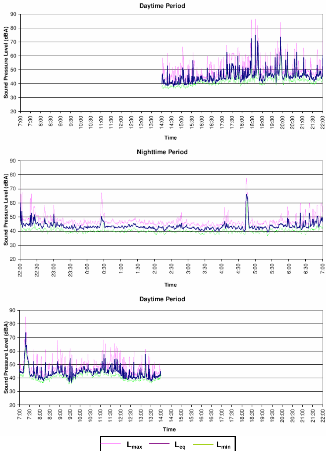
Figure I-2: Monitored 1-Minute L_{eq} Baseline Sound Values Opposite Residence 1, November 8–9, 2005
