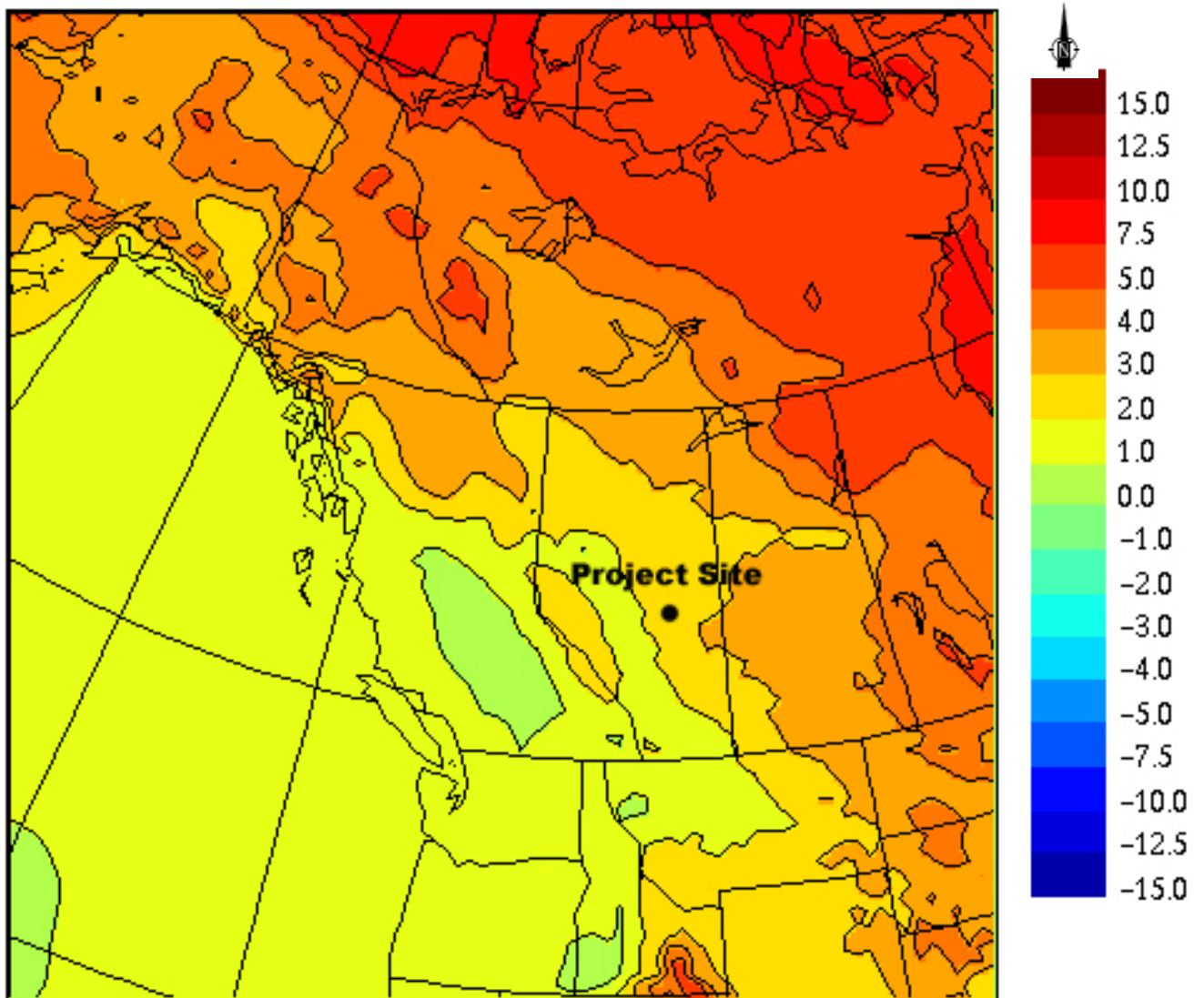
Figure 2.7-1: Estimated Surface Temperature Variance (2 m) in the Project Area (°C): 1975–1984 vs. 2040–2049 Generated by CGCM3 Assuming IPCC Scenario IS92a
