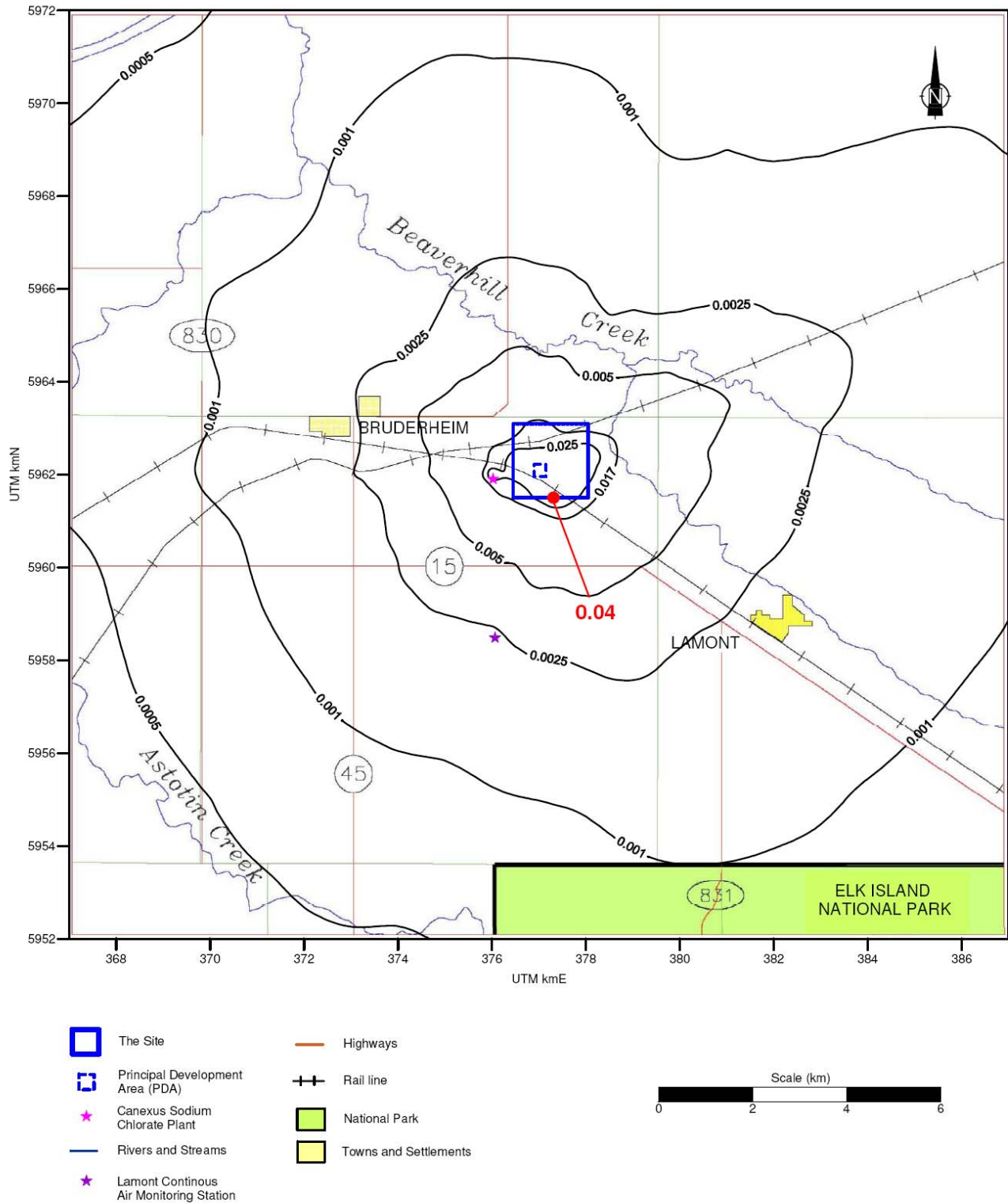
Figure 2.5-13: Isopleths of Predicted Annual Average PAI Values (keq H + (ha·y)) associated with Emissions from the Project plus the Canexus Sodium Chlorate Plant
