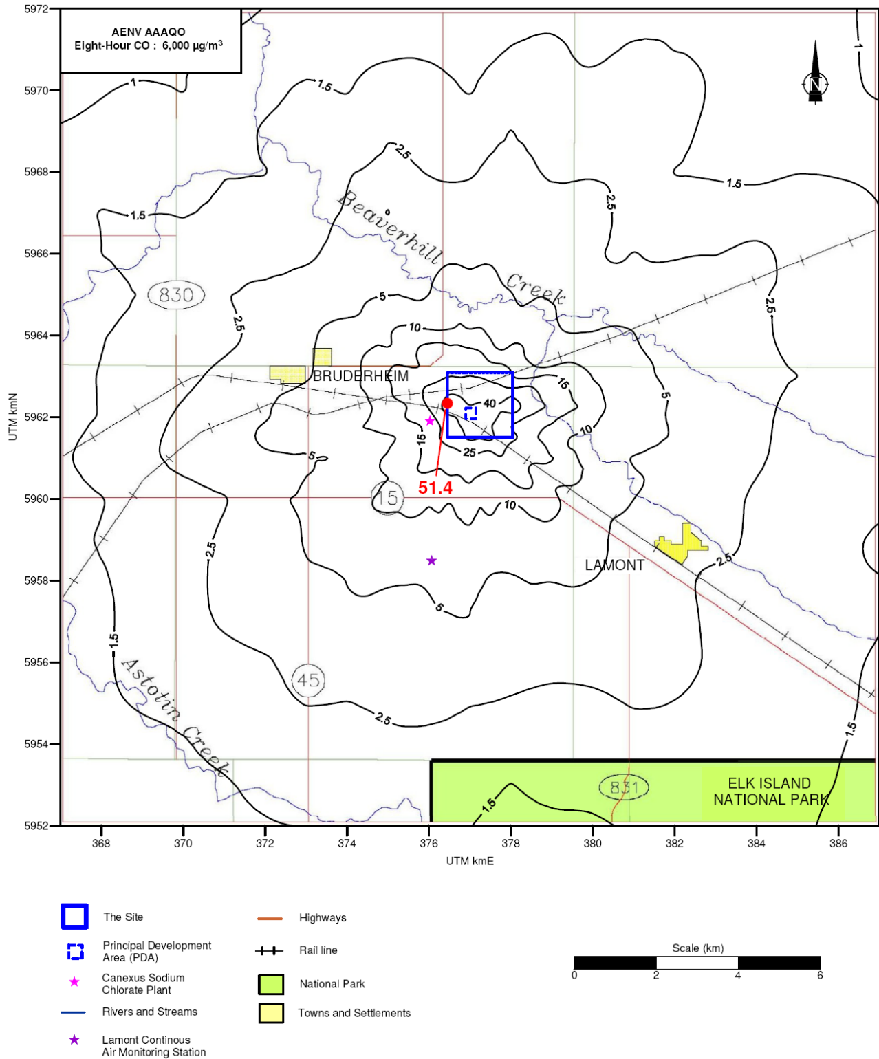
Figure 2.5-3: Isopleths of Maximum Predicted 8-Hour Average Ground-level CO Concentrations ( \mu\text{g}/\text{m}^3 ) associated with Emissions from the Project plus the Canexus Sodium Chlorate Plant
