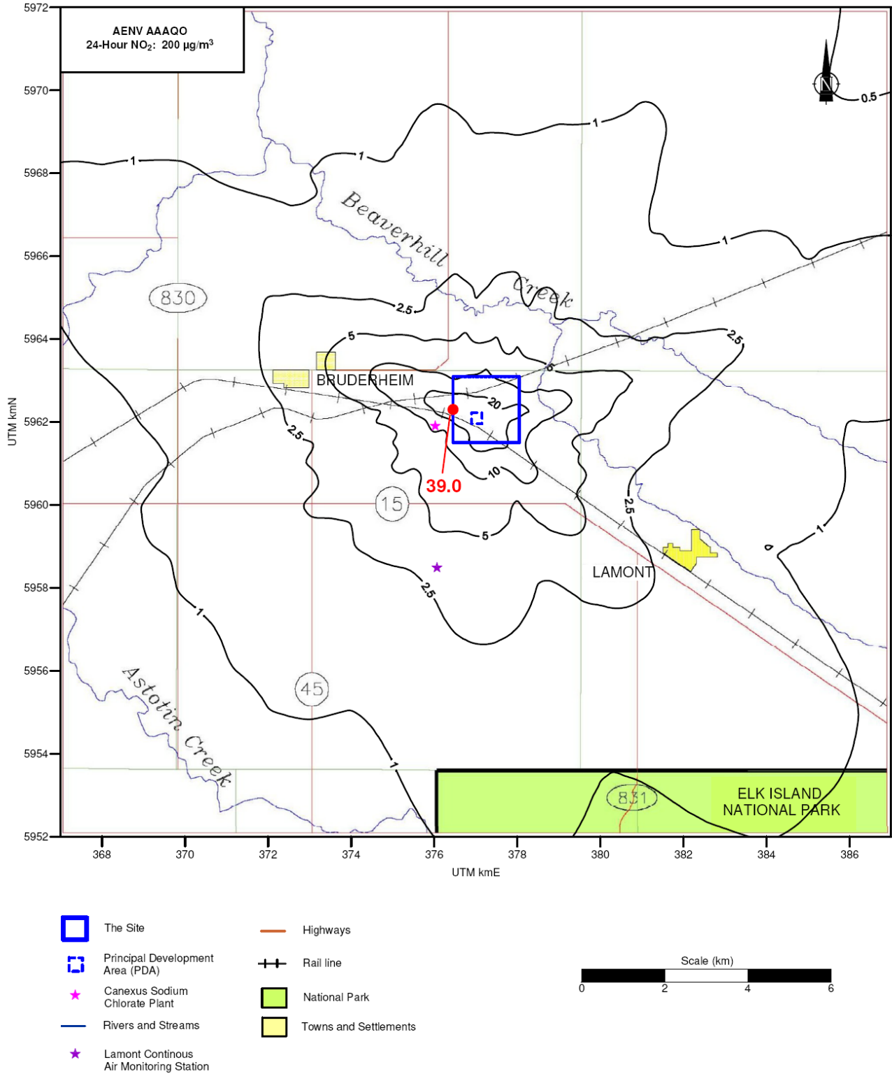
Figure 2.5-7: Isopleths of Maximum Predicted Daily Average Ground-level NO 2 Concentrations (µg/m 3 ) associated with Emissions from the Project plus the Canexus Sodium Chlorate Plant
