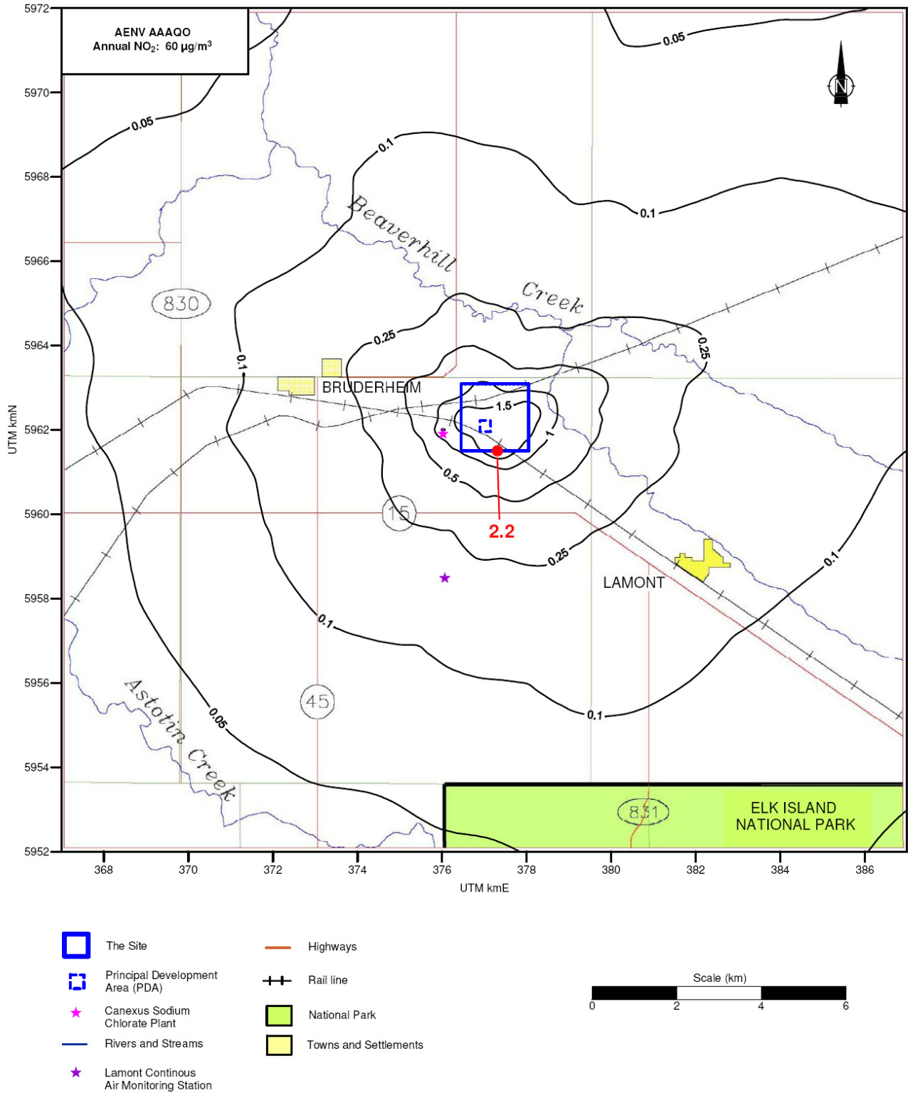
Figure 2.5-8: Isopleths of Maximum Predicted Annual Average Ground-level NO 2 Concentrations (µg/m 3 ) associated with Emissions from the Project plus the Canexus Sodium Chlorate Plant
