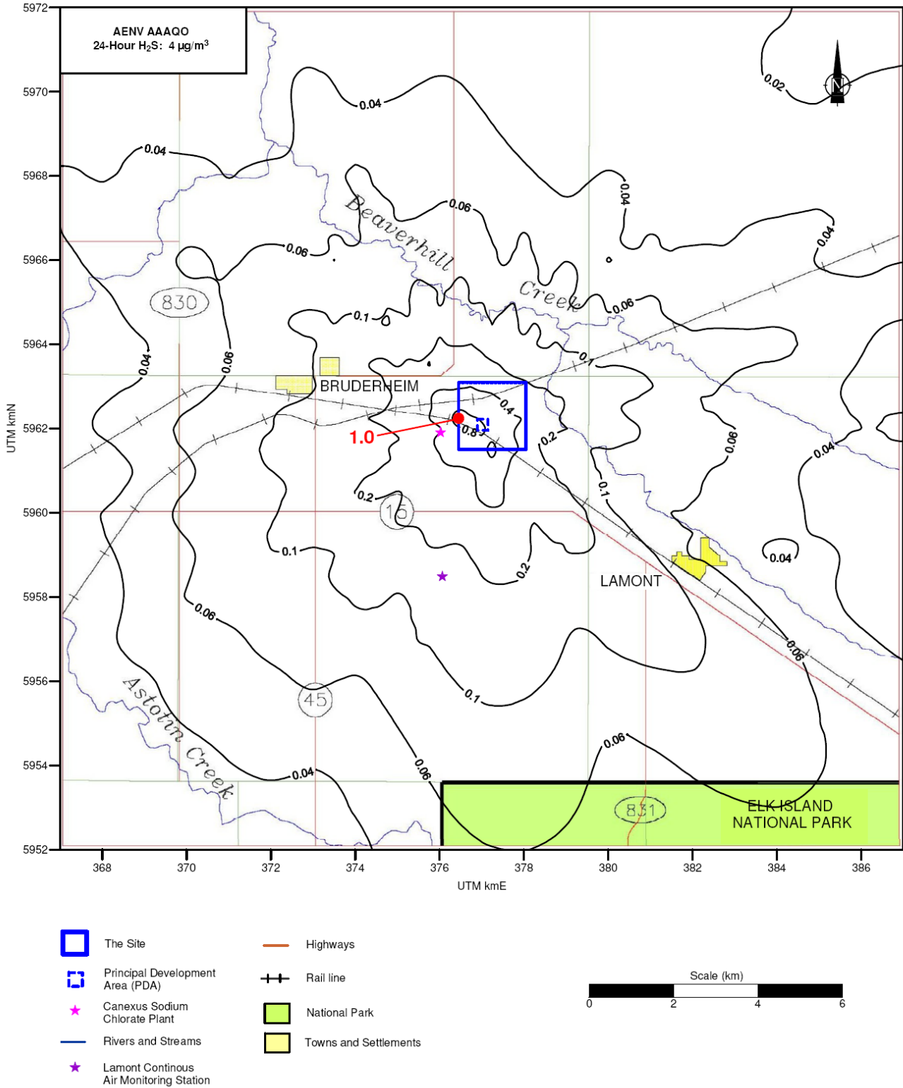
Figure 2.5-5: Isopleths of Maximum Predicted Daily Average Ground-level H 2 S Concentrations (µg/m 3 ) associated with Emissions from the Project plus the Canexus Sodium Chlorate Plant
