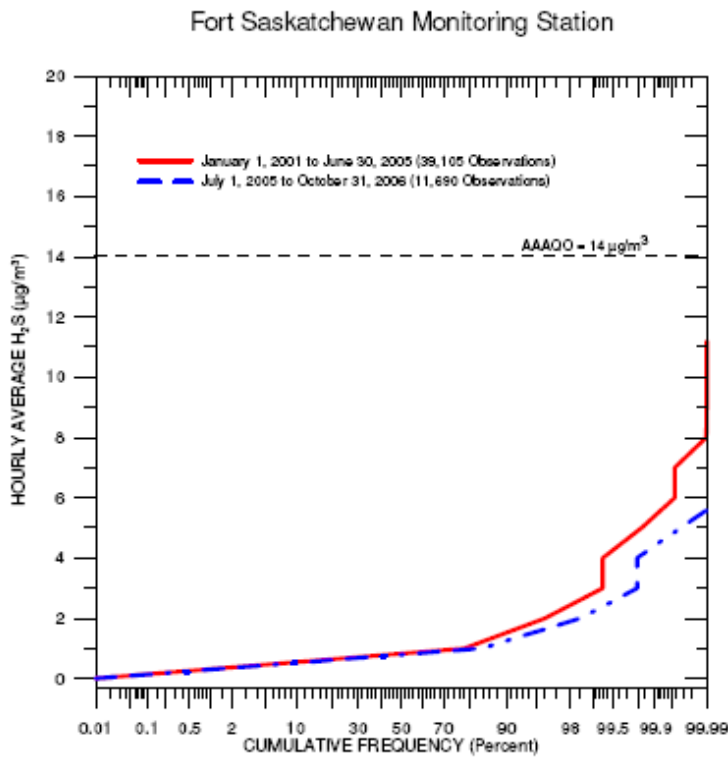
Figure 2.4-3: Cumulative Frequency Distributions of Hourly Average H 2 S Concentrations (µg/m 3 ) Observed over the Indicated Periods at the Lamont and Fort Saskatchewan Air Quality Monitoring Stations
