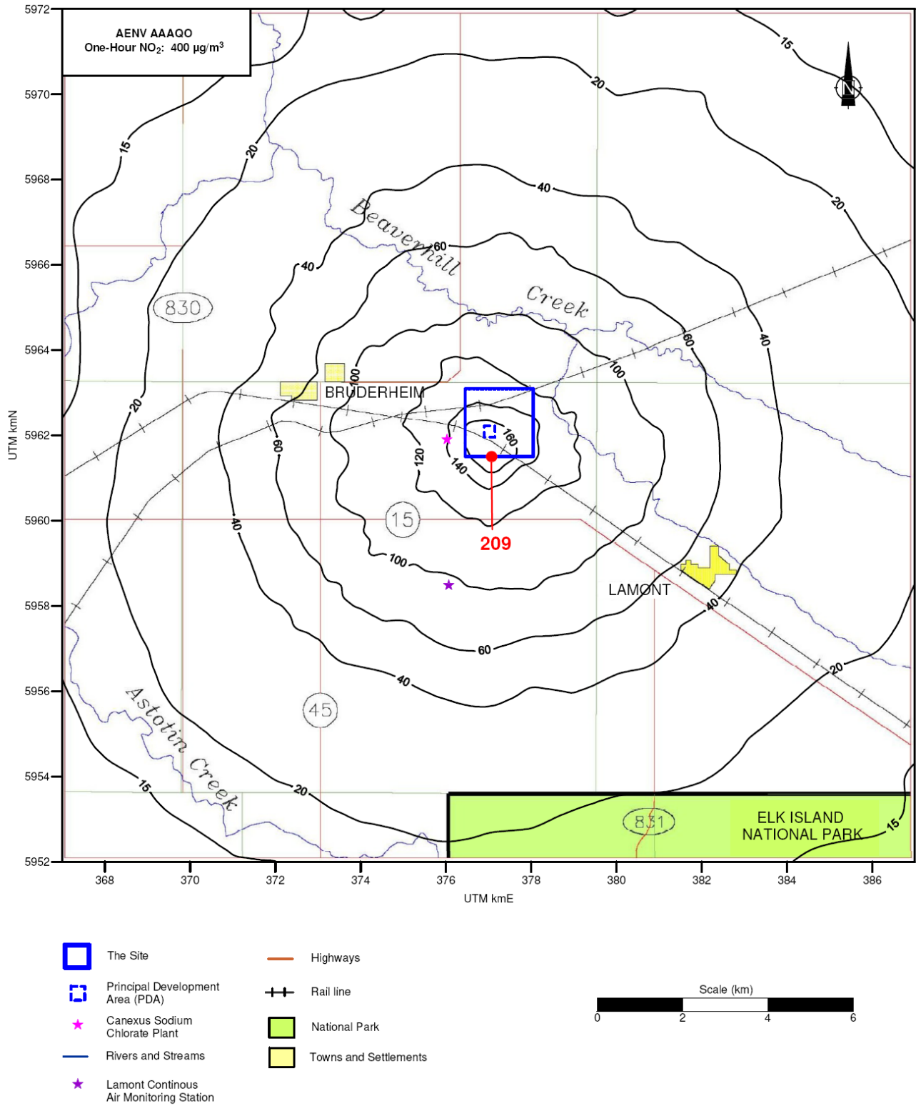
Figure 2.5-6: Isopleths of Maximum Predicted Hourly Average Ground-level NO 2 Concentrations (µg/m 3 ) associated with Emissions from the Project plus the Canexus Sodium Chlorate Plant
