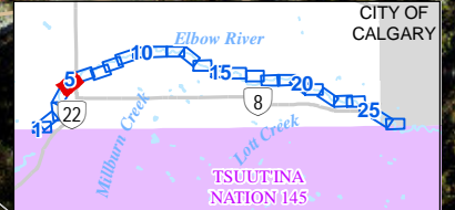
Bull Trout HSI Map for Elbow River (Spawning Life Stage)
