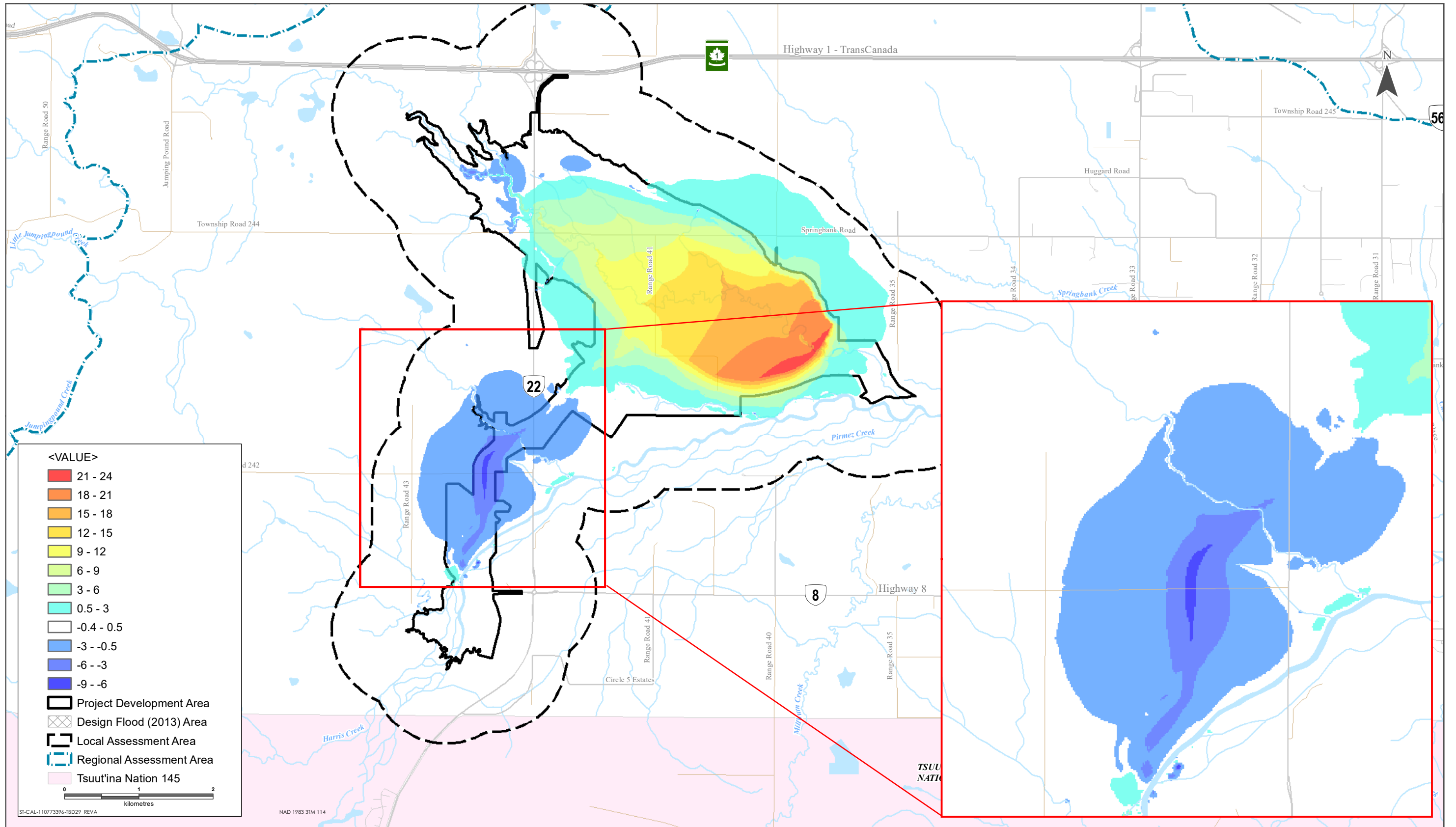
Simulated Net Change in Head for the PPX1/EEX1 Sensitivity Scenario 1 at Timestep 650 with Conservative Loading Applied (revised from Round 2 AEP, IR42, Appendix 42-1, Figure E1.1)
