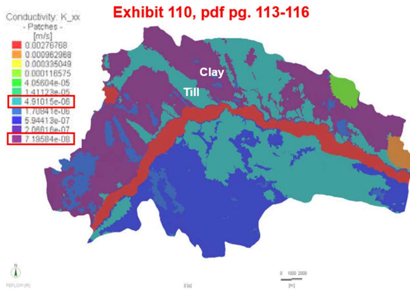
Figure 4-5 Hydraulic Conductivity Distribution in Layer 1
