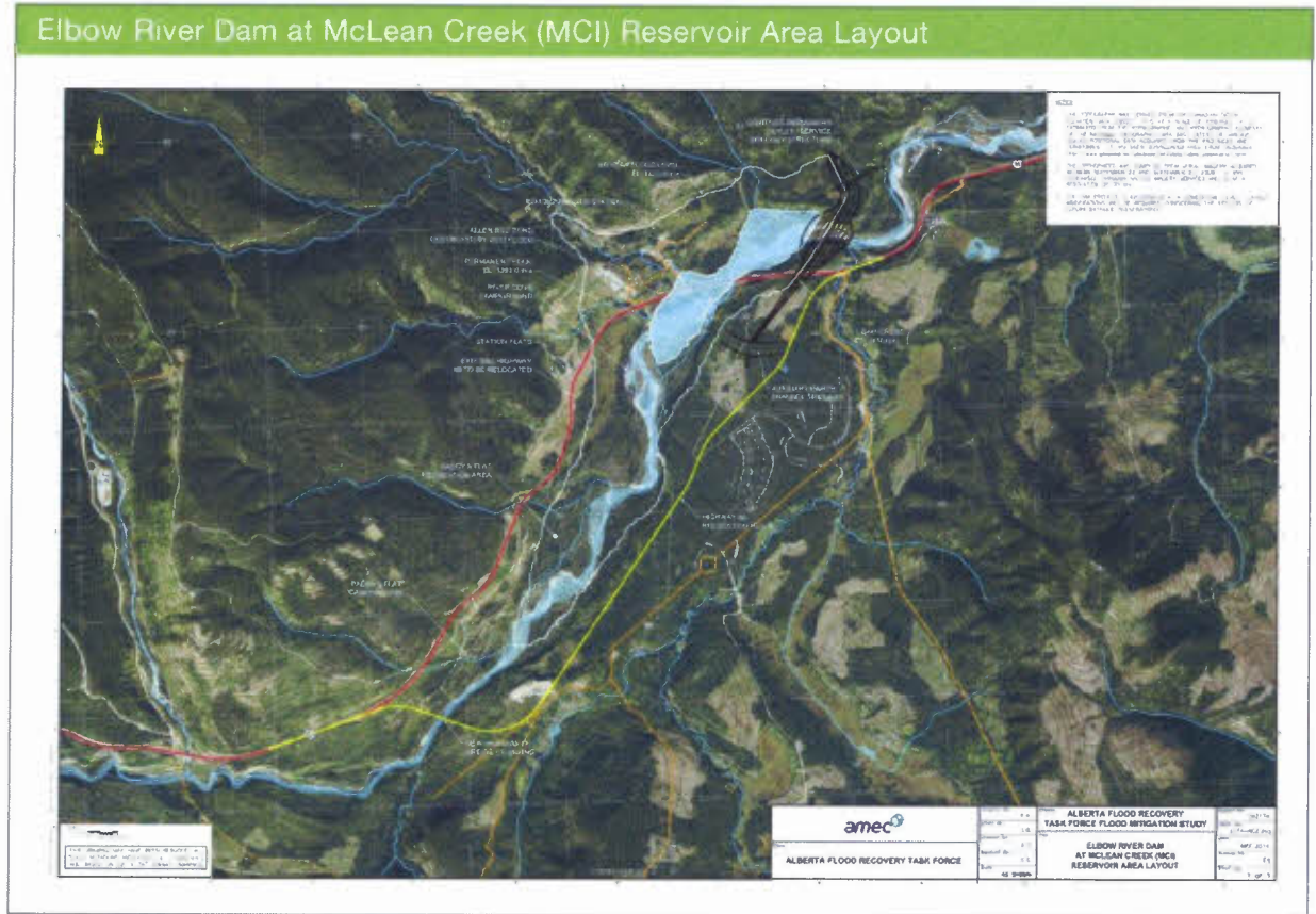
Figure 1 Location and reservoir area of the Elbow River Dam at McLean Creek (MCI)
